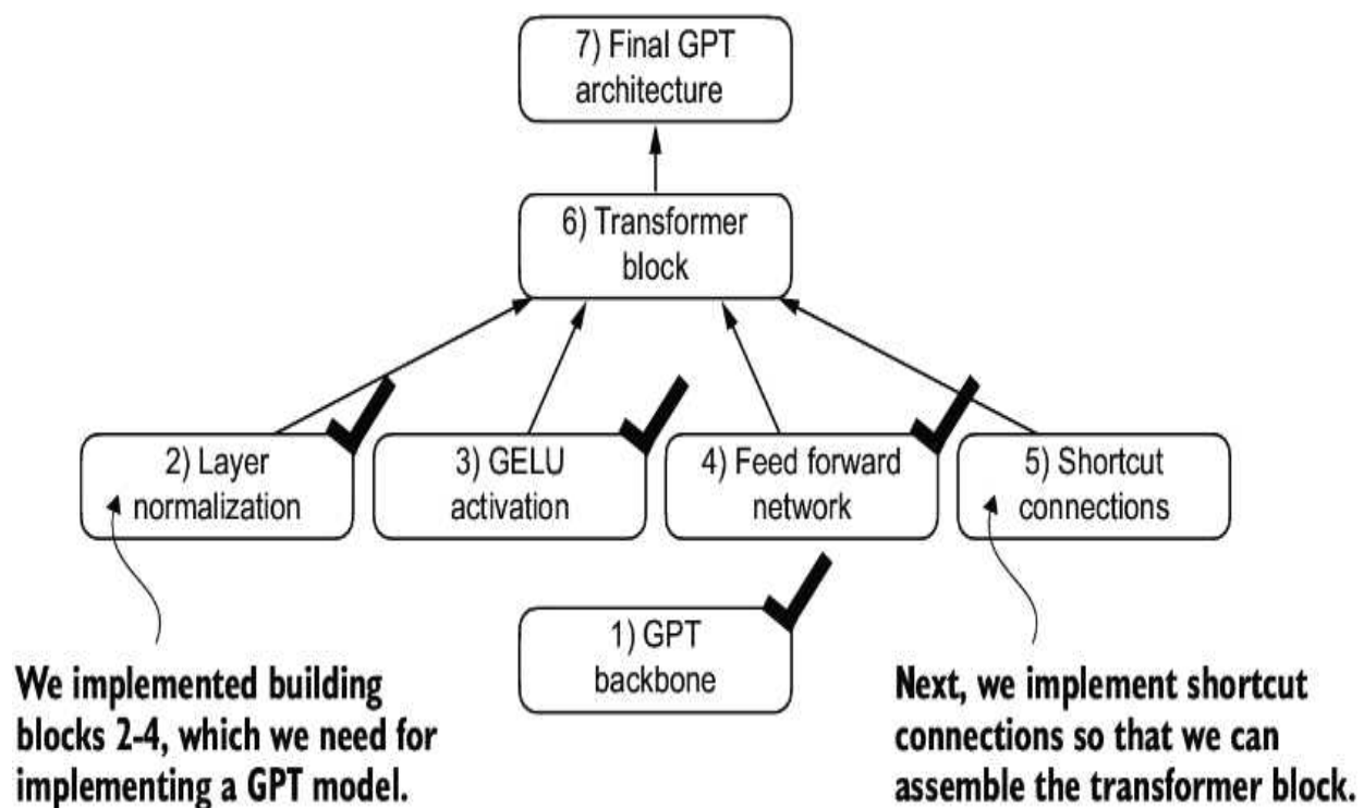
Figure 4.11 The building blocks necessary to build the GPT architecture. The black checkmarks indicating those we have already covered.
