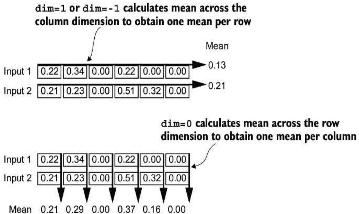
Figure 4.6 An illustration of the dim parameter when calculating the mean of a tensor. For instance, if we have a two-dimensional tensor (matrix) with dimensions [rows, columns], using dim=0 will perform the operation across rows (vertically, as shown at the bottom), resulting in an output that aggregates the data for each column. Using dim=1 or dim=-1 will perform the operation across columns (horizontally, as shown at the top), resulting in an output aggregating the data for each row.
