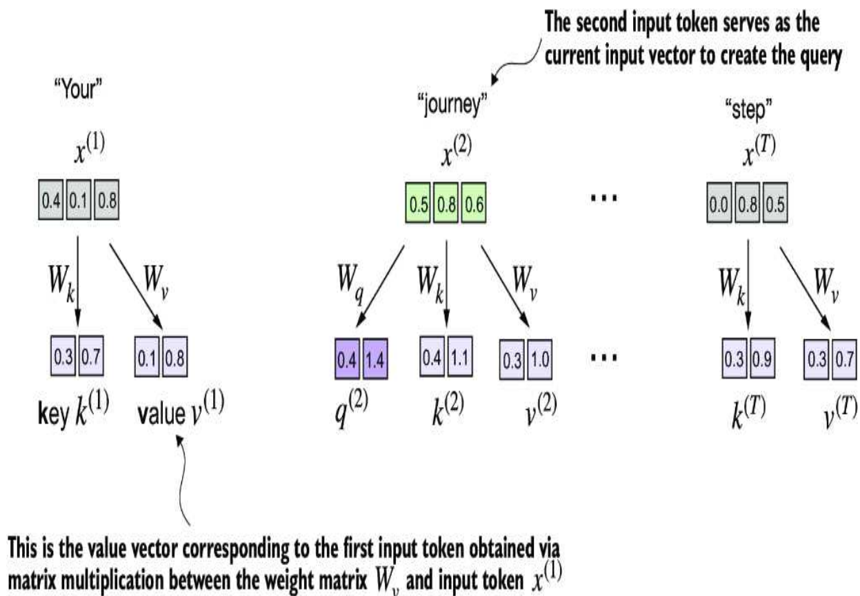
Figure 3.14 In the first step of the self-attention mechanism with trainable weight matrices, we compute query (q), key (k), and value (v) vectors for input elements x . Similar to previous sections, we designate the second input, x^{(2)} , as the query input. The query vector q^{(2)} is obtained via matrix multiplication between the input x^{(2)} and the weight matrix W_q . Similarly, we obtain the key and value vectors via matrix multiplication involving the weight matrices W_k and W_v .
