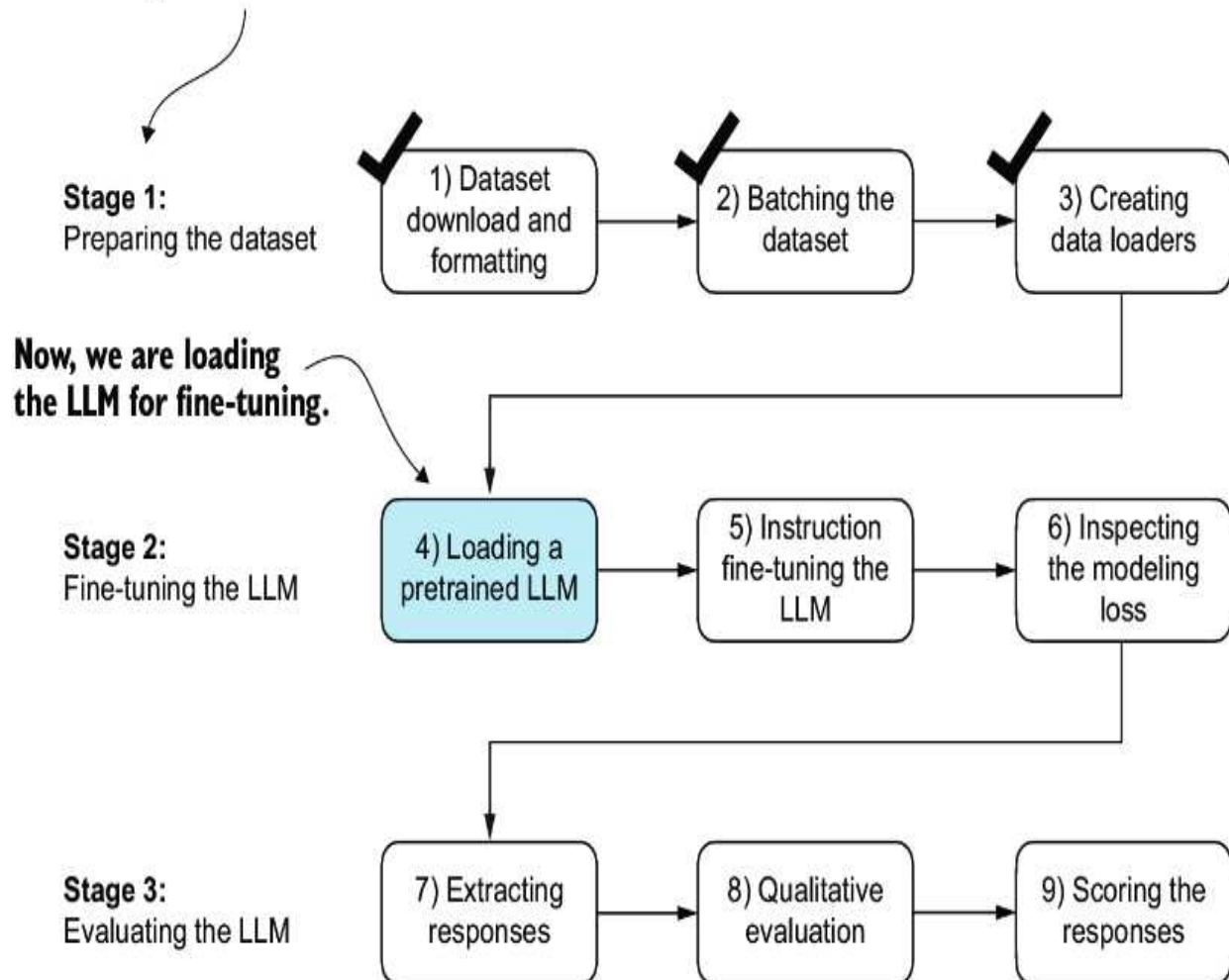
Figure 7.15 The three-stage process for instruction fine-tuning an LLM. After the dataset preparation, the process of fine-tuning an LLM for instruction-following begins with loading a pretrained LLM, which serves as the foundation for subsequent training.
